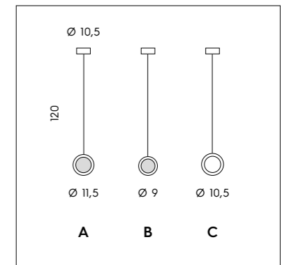
SP 7/330 A - B - C 6W STRIP LED 800 lumen - 3000K CE IP20
