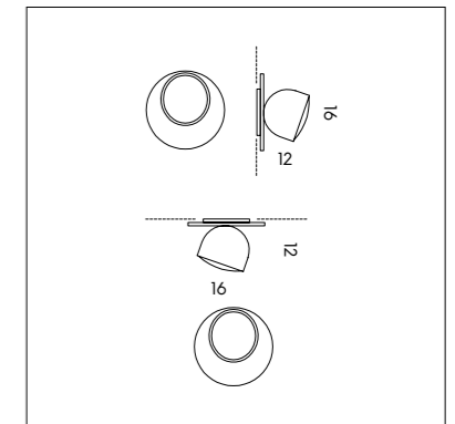
LS 4/310 7W LED 765 lumen - 3000K CE IP20
